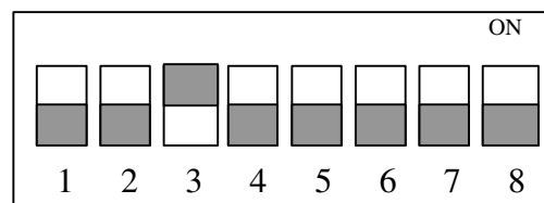
Slave Address 4
