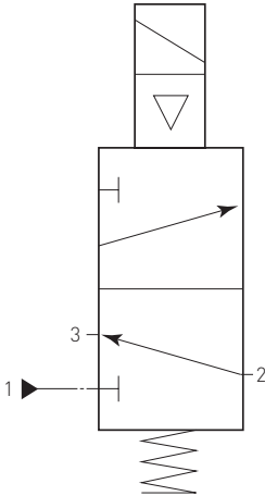
FIGURE 1 - SPRING RETURN VALVE 3/2 WAY
