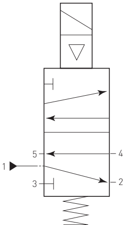
FIGURE 2 - SPRING RVETURN VALVE 5/2 WAY
